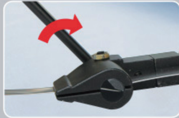
RST-220, 240 CUTTER DETAIL (PULL AND PRESS TYPE CUTTER LEVER)
