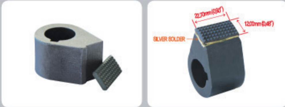
GRIPPER DETAIL (BRAZED TUNGSTEN CARBIDE BY SILVER SOLDER)
