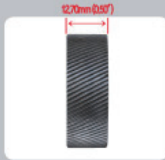
EFT-190 FEEDWHEEL DETAIL (TUNGSTEN CARBIDE)
